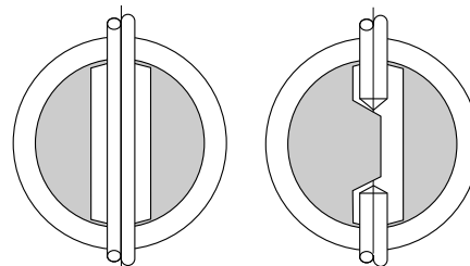
Competitor one-piece stem K-LOK® two-piece stem
